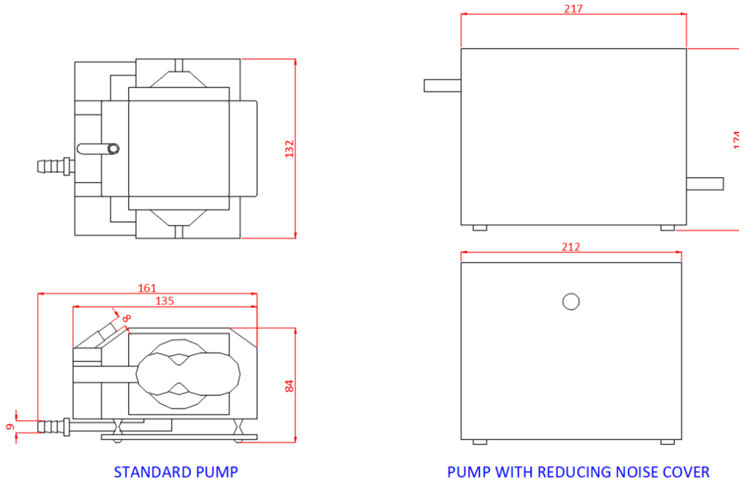
STANDARD PUMP
